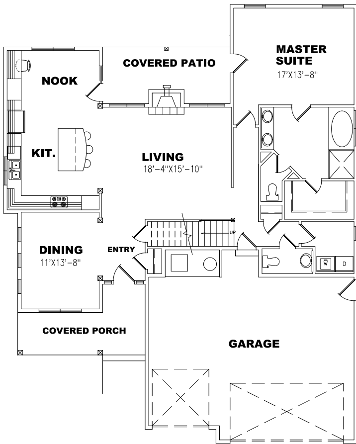
1586 SQ' MAIN FLOOR
